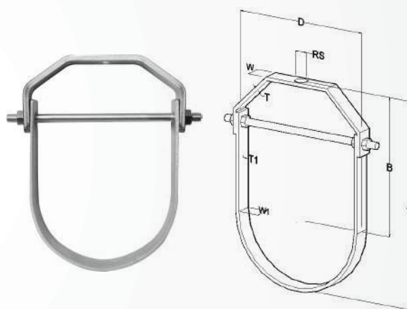
Heavy pipe suspended support
